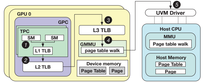
Fig. 1. UVM-managed Multi-GPU overview
