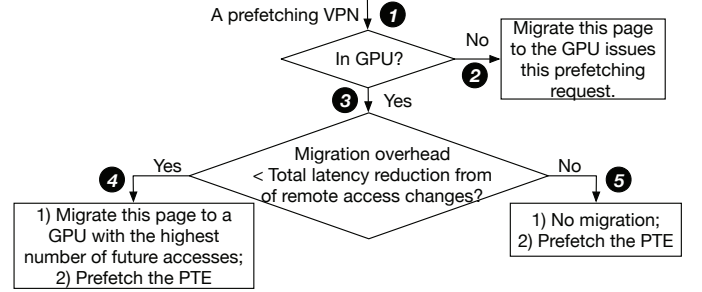
Fig. 12. Coordination logic
