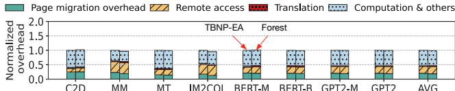
Fig. 5. Performance breakdown normalized to TBNP-EA
