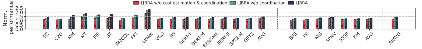
Fig. 19. Impact of each LIBRA design component on overall performance (left: regular benchmarks, middle: irregular benchmarks, right: overall average)
