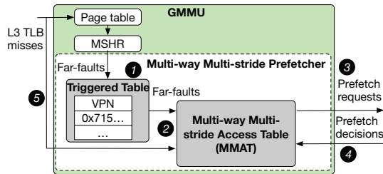
Fig. 9. Multi-way multi-stride prefetcher design
