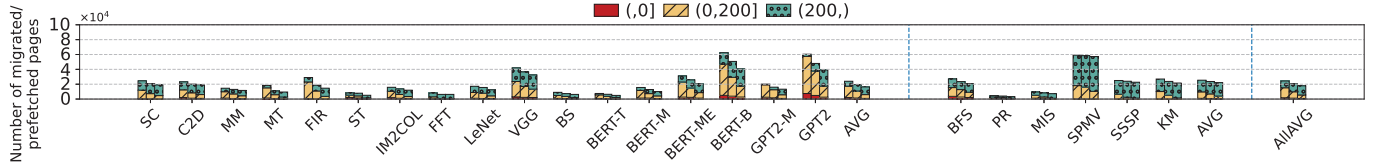
Fig. 20. Total remote access changes for migrated/prefetched pages (left: regular benchmarks, middle: irregular benchmarks, right: overall average). The bars for each benchmark, from left to right, represent LIBRA w/o cost estimation & coordination, LIBRA w/o coordination, and LIBRA
