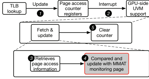
Fig. 11. Access counter update logic
