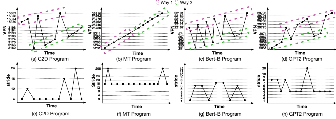
Fig. 4. VPN accesses of a SM: (a) C2D, (b) MT, (c) BERT-B, (d) GPT-2. VPN access strides of a way of a SM: (e) C2D, (f) MT, (g) BERT-B, (h) GPT-2.
