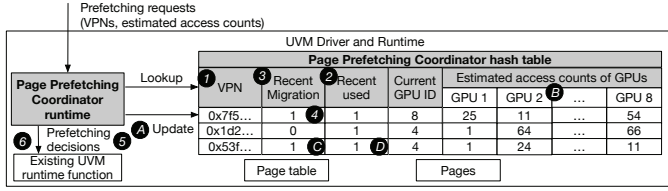
Fig. 13. Page prefetching coordinator design
