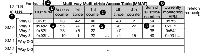
Fig. 10. Multi-way Multi-stride Access Table
