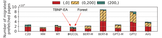
Fig. 6. Total remote access changes for all migrated/prefetched pages.
