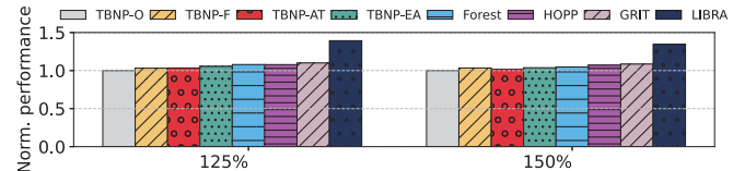
Fig. 24. Memory oversubscription performance
