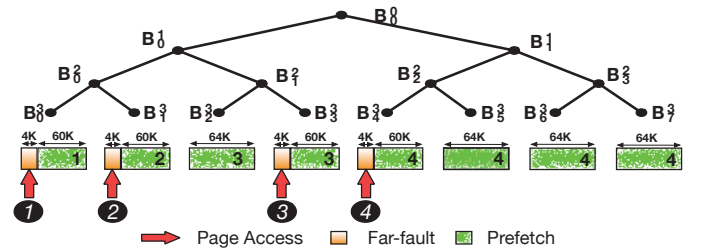
Fig. 2. NVIDIA tree-based neighborhood prefetcher [21]
