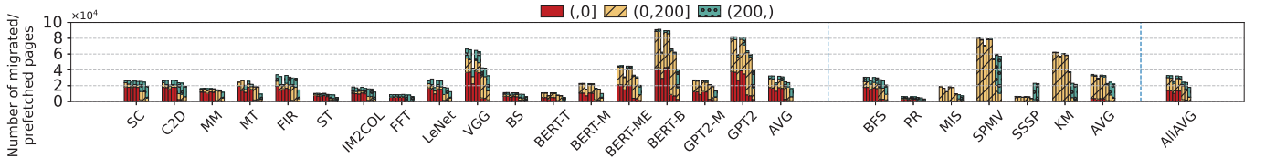
Fig. 17. Total remote access changes for all migrated/prefetched pages (left: regular benchmarks, middle: irregular benchmarks, right: overall average). The bars for each benchmark, from left to right, represent TBNP-O, TBNP-F, TBNP-AT, TBNP-EA, Forest, HOPP, GRIT, and LIBRA
