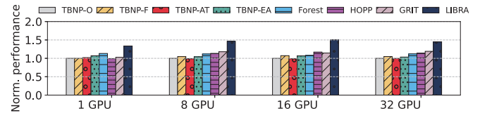
Fig. 23. Average performance with 1, 8, 16, and 32 GPUs
