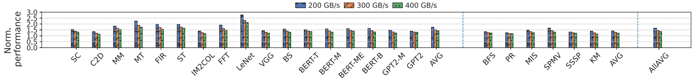
Fig. 22. Performance with 200 GB/s, 300 GB/s, and 400 GB/s NVLink Bandwidth (Left: Regular benchmarks Middle: Irregular benchmarks Right: Overall Average Results)
