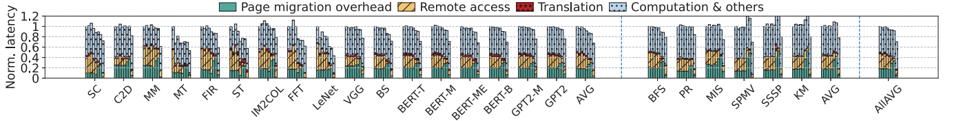
Fig. 15. Performance breakdown normalized to TBNP-O (left: regular benchmarks, middle: irregular benchmarks, right: overall average). The bars for each benchmark, from left to right, represent TBNP-O, TBNP-F, TBNP-AT, TBNP-EA, Forest, HOPP, GRIT, and LIBRA
