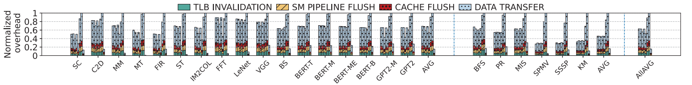
Fig. 16. Breakdowns of page migration overhead normalized to GRIT (left: regular benchmarks, middle: irregular benchmarks, right: overall average). The bars for each benchmark, from left to right, represent TBNP-O, TBNP-F, TBNP-AT, TBNP-EA, Forest, HOPP, GRIT, and LIBRA
